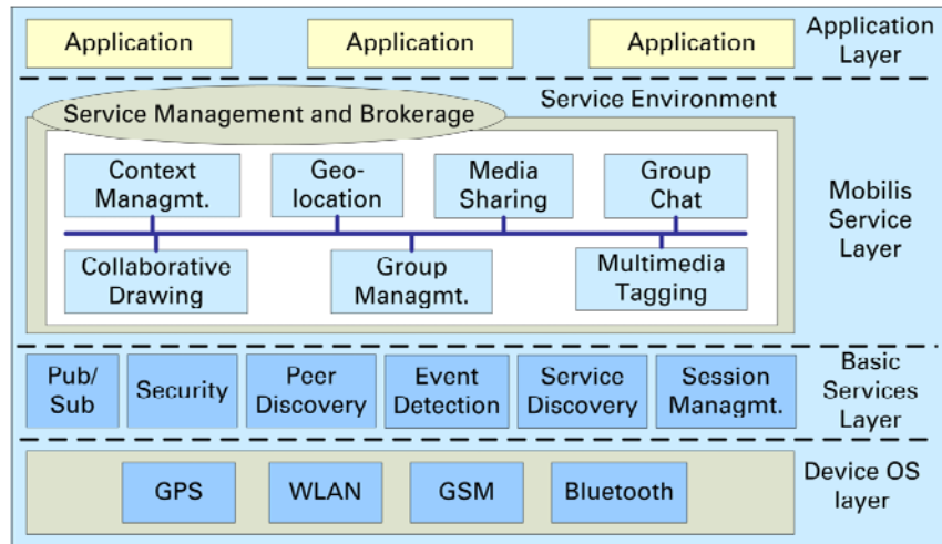
FIGURE 1: MOBILIS REFERENCE ARCHITECTURE
