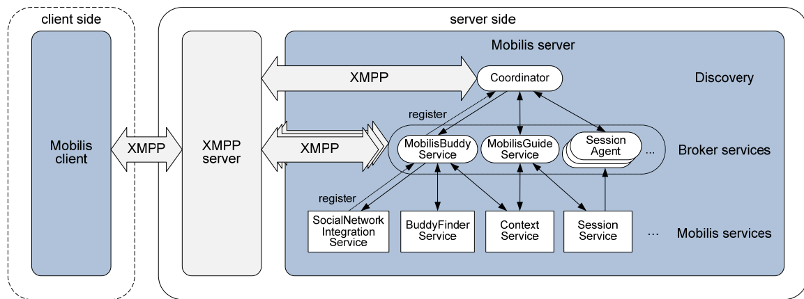
FIGURE 3: XMPP-BASED ARCHITECTURE
